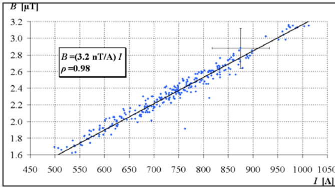
Figure 4. Relationship between measured induction and line current for a single line case (n. 356, 380 kV).
