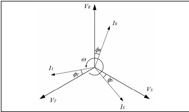
Figure 1. Phasors V - I diagram.
