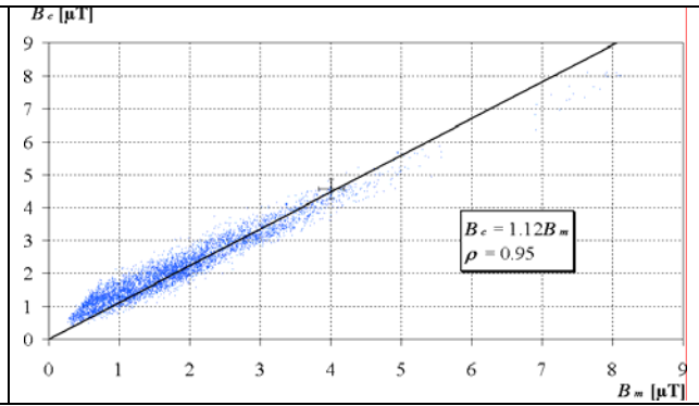
Figure 5. Relationship between induction measured ( B_m ) in proximity to a double line and that calculated by Phidel ® ( B_c ).
