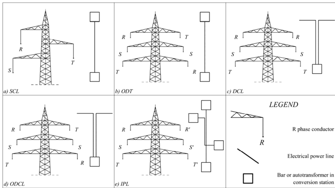
Figure 3. Schematic representation of power line typologies.
