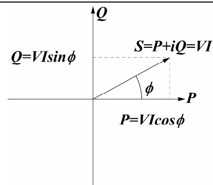
Figure 2. Scalar P - Q diagram.
