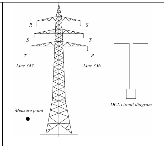
Figure 6b. Disposition of the phases on a pylon of the 347-356 DCL and relative circuit diagram.
