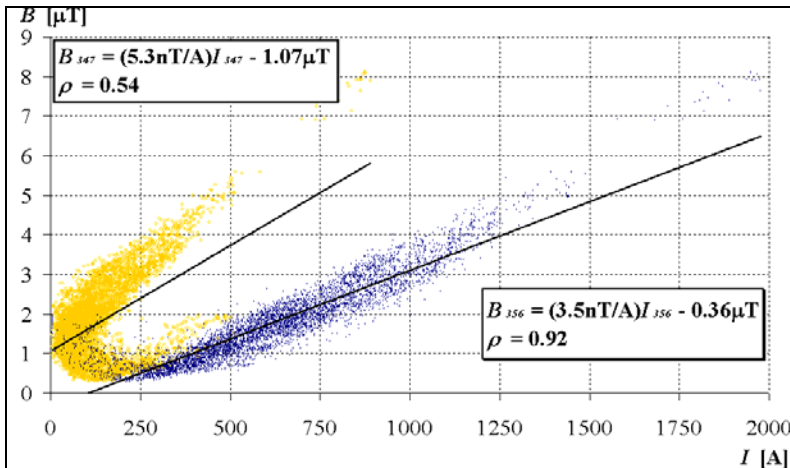
Figure 6a. Magnetic induction in function of current for lines 347 (orange dots) and 356 (blue dots).
